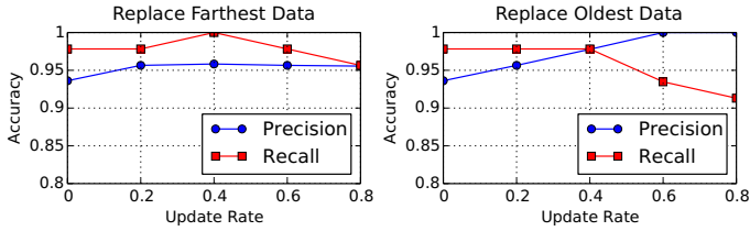
Figure 13: Accuracy of by the classifier with the auto-calibration. The update rate means how many portions of the training data set is replaced with the new data (e.g. update rate = 0.4 means 40% of the training set should be replaced with the new data for each auto-calibration).
