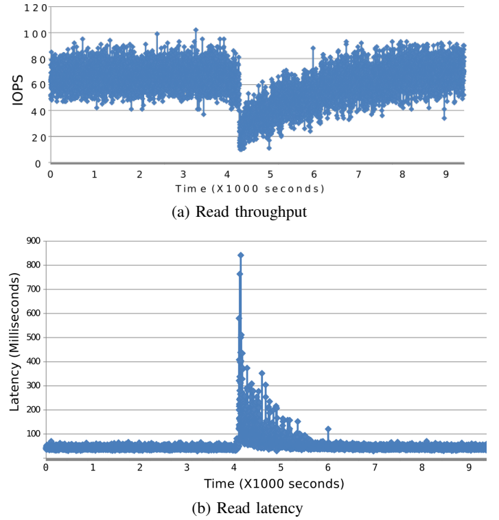
Fig. 13: Throughput (IOPS) and latency (milliseconds) of read requests for data on a server before and after it fails. The failure occurs at about the 4100th second.
