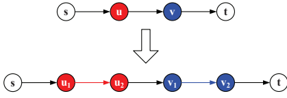
Fig. 2. An example of graph transformation
