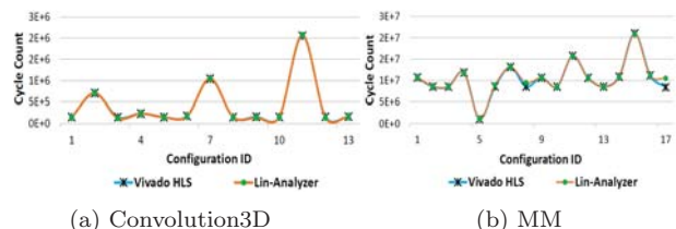
Figure 3: Accuracy of Lin-Analyzer with loop unrolling and pipelining pragmas compared to Vivado HLS
